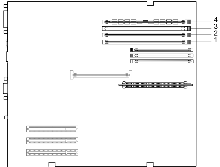
Figure: DRAM DIMM Slots
